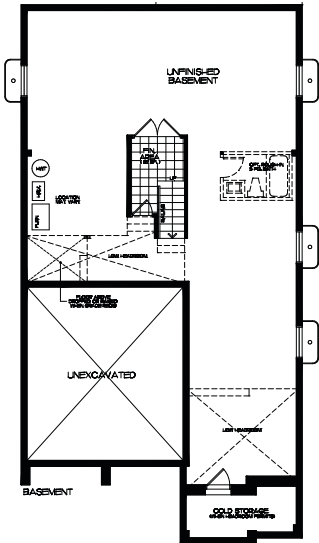
BASEMENT - ELEV. A TYPE BH-415
