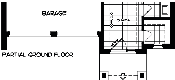
PARTIAL GROUND FLOOR - ELEV. B TYPE BH-415 G.F.A. = 3249 sf. (plus 52 sf. fin. basement)
