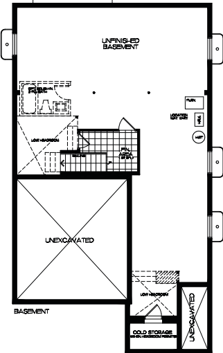
BASEMENT - ELEV. A TYPE BH-412
