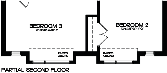
PARTIAL SECOND FLOOR - ELEV. B TYPE BH-416
