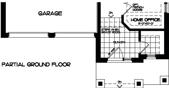
PARTIAL GROUND FLOOR - ELEV. B TYPE BH-416 G.F.A. = 3379 sf. (plus 96 sf. fin. basement)
