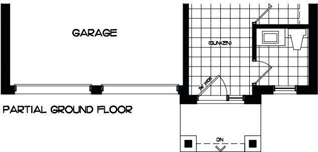
PARTIAL GROUND FLOOR - ELEV. B TYPE BH-411 G.F.A. = 2592 sf. (plus 73 sf. fin. basement)
