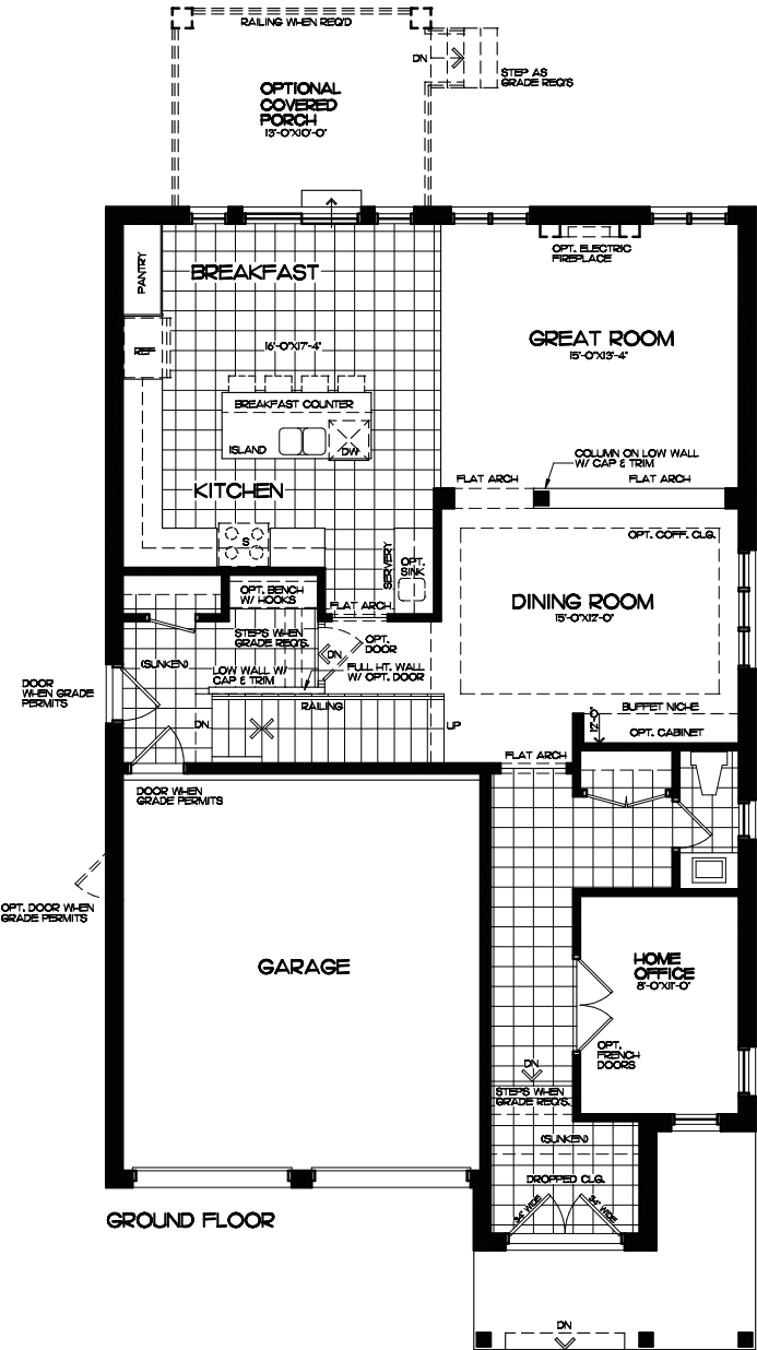
PARTIAL GROUND FLOOR - ELEV. B TYPE BH-412 G.F.A. = 2737 sf. (plus 59 sf. fin. basement)
