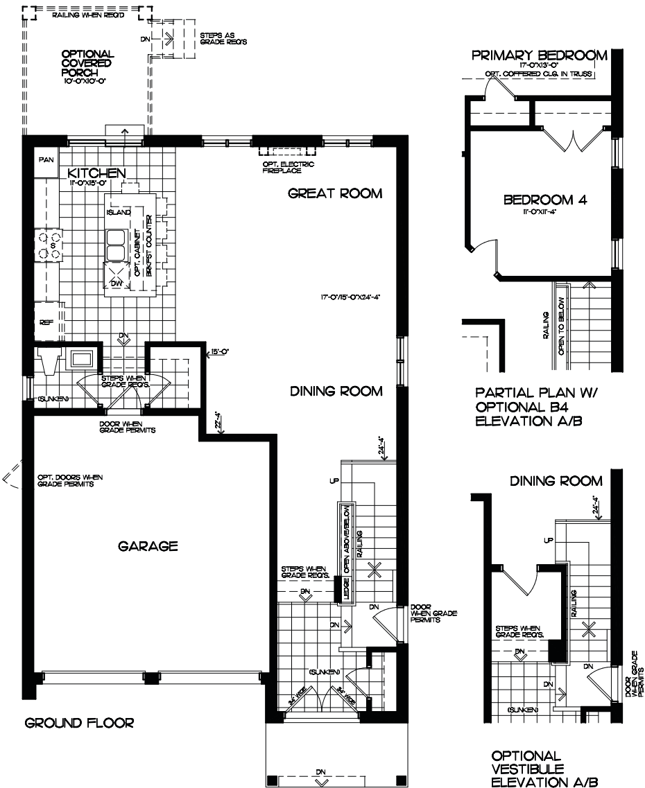
GROUND FLOOR - ELEV. A TYPE BH-381 G.F.A. = 2213 sf. (plus 85 sf. fin. basement)
