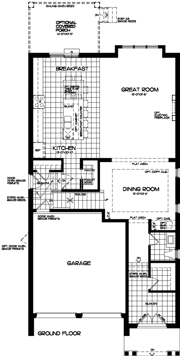
GROUND FLOOR - ELEV. A TYPE BH-386 G.F.A. = 2869 sf. (plus 83 sf. fin. basement)
