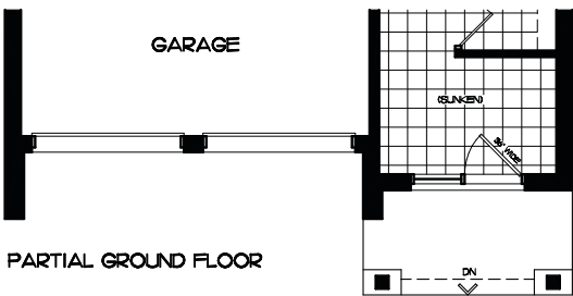
PARTIAL GROUND FLOOR - ELEV. B TYPE BH-386 G.F.A. = 2867 sf. (plus 83 sf. fin. basement)
