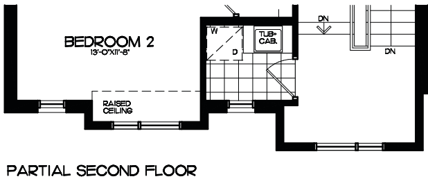
PARTIAL SECOND FLOOR - ELEV. B TYPE BH-381
