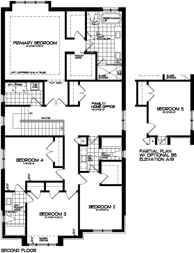
PARTIAL SECOND FLOOR - ELEV. B TYPE BH-386
