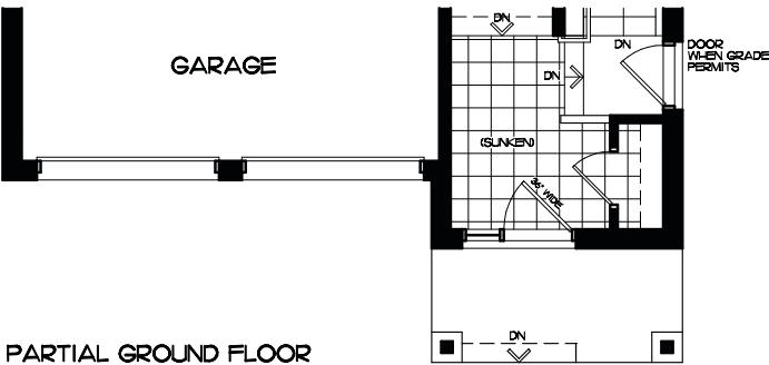
PARTIAL GROUND FLOOR - ELEV. B TYPE BH-381 G.F.A. = 2212 sf. (plus 85 sf. fin. basement)
